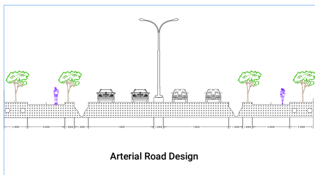
Figure 3. Road Designs
