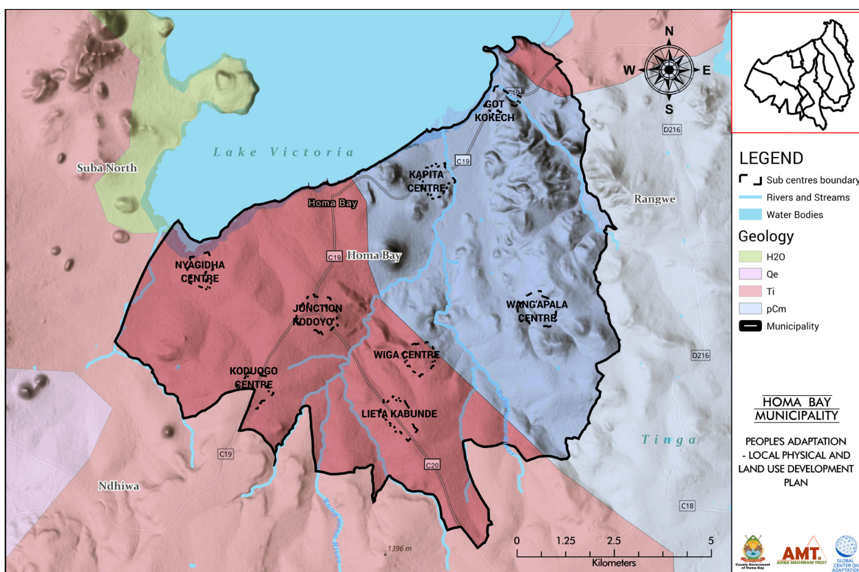
Map 7. Geological Formations
